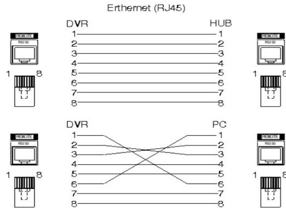
[Fig. 5-9 Straight-through & Crossover Cable]
